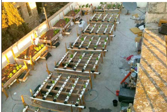
FIGURE 4.17 Multiple aquaponic systems on a rooftop
