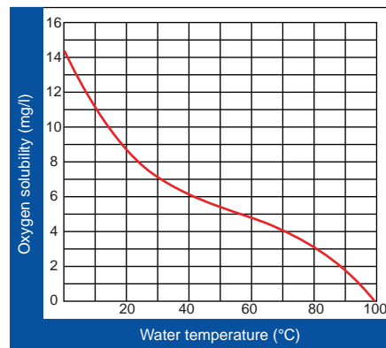
FIGURE 3.4 Oxygen solubility in water at different temperatures
