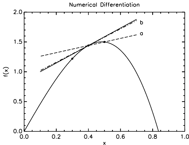
Figure 2: The centered derivative approximation works best.
