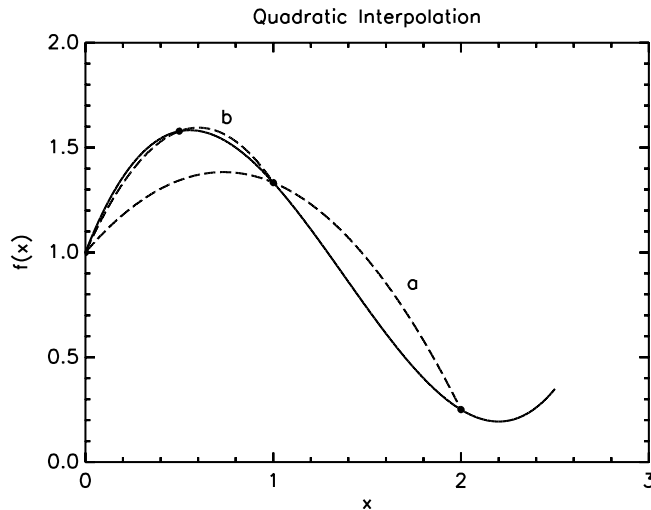
Figure 6: Quadratic interpolation follows the curves better if the curvature doesn't change sign.
