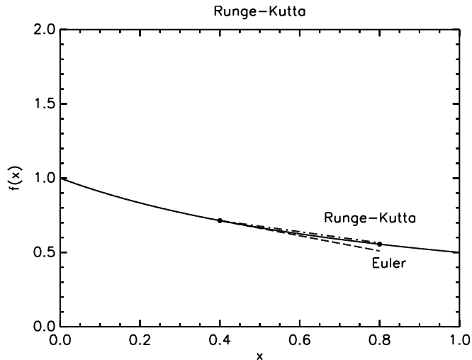
Figure 7: Runge-Kutta anticipates curving and beats Euler.
