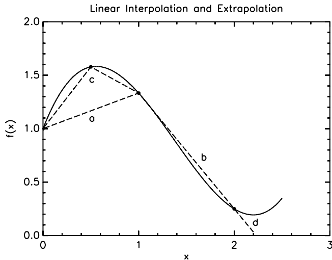
Figure 5: Linear interpolation only works well over intervals where the function is straight.
