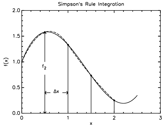
Figure 4: Fitting parabolas (Simpson's Rule) works better.
