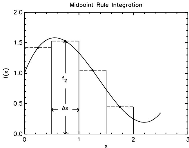
Figure 3: The midpoint rule works OK if the function is nearly straight across each interval.
