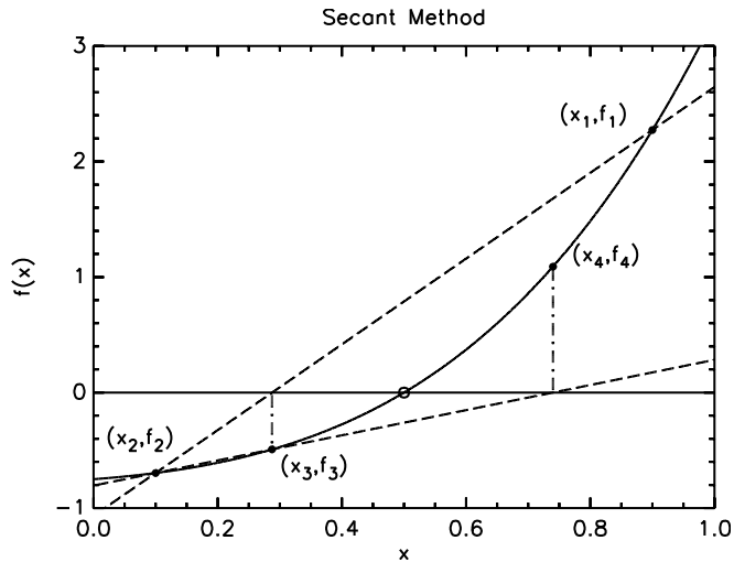
Figure 1: The sequence of approximate points in the secant method.
