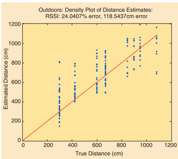
Fig. 6 RSSI Density Plot for outdoor data
