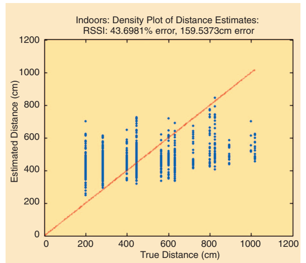
Fig. 4 RSSI Density Plot for indoor data
