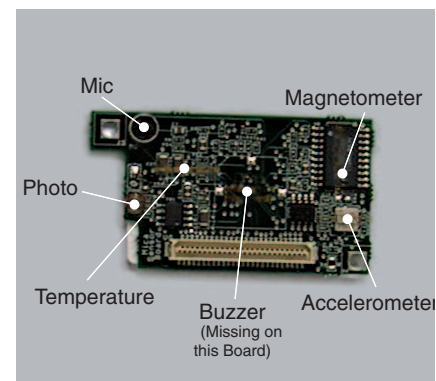
Fig. 1 The Mica Sensorboard
