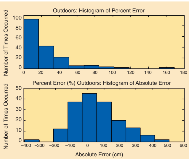
Fig. 5 Percent and Absolute Error Plots for outdoor data
