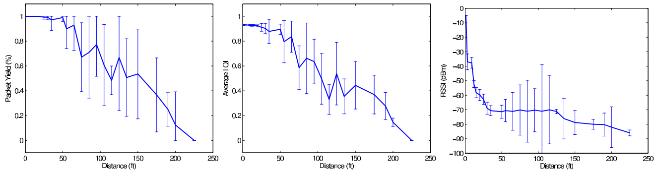
Fig. 5. Packet yield (left), link quality indicator (LQI, center), and received signal strength (RSSI, right) outdoors with the Telos mote and internal antenna. The results are averaged over 10 receivers co-located. From 75-110 feet, a dip in the terrain yields more erratic readings and wider variation in RSSI.
