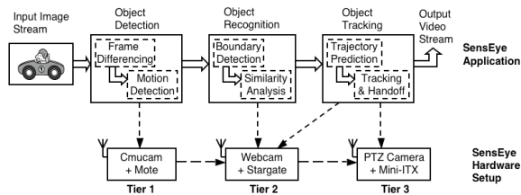
Figure 2: Software architecture of SensEye .
